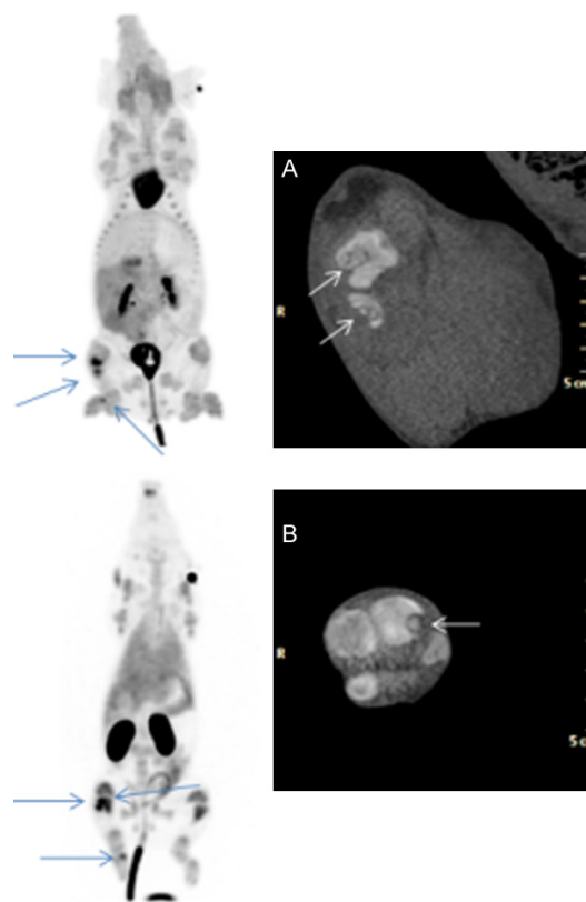
Figure 5. Left: [ 18 F]FDG (maximal intensity projection (MIP), upper) and [ 99m Tc]IL8 (MIP lower) uptake in pig 4 with 3 osteomyelitis lesions in the right hind limb as indicated by arrows. Right: CT (bone window) of A: osteomyelitis in proximal tibia and fibula, and of B: osteomyelitis in the third metatarsal bone. All OM having formed sequesters and fistulous tracts. The lesions are marked with an arrow. To the right in the CTs is shown a size bar (5 cm).
