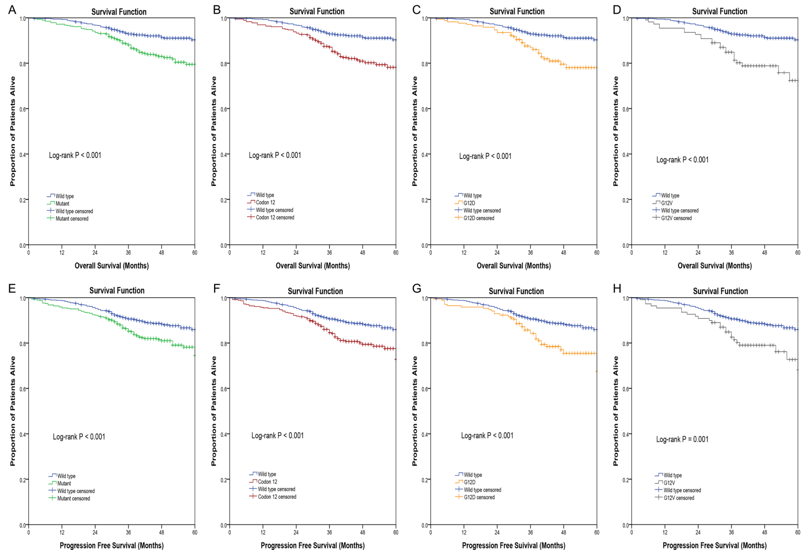
Figure 2. Kaplan-Meier curves of colorectal cancer patients according to KRAS mutation status. Overall survival in months according to (A) KRAS mutation status, (B) KRAS codon 12 mutation status, (C) KRAS G12D mutation status, (D) KRAS G12V mutation status. Progression free survival in months according to (E) KRAS mutation status, (F) KRAS codon 12 mutation status, (G) KRAS G12D mutation status, (H) KRAS G12V mutation status. Log rank test was used to compare the survival distributions. P < 0.05 was considered significant.
