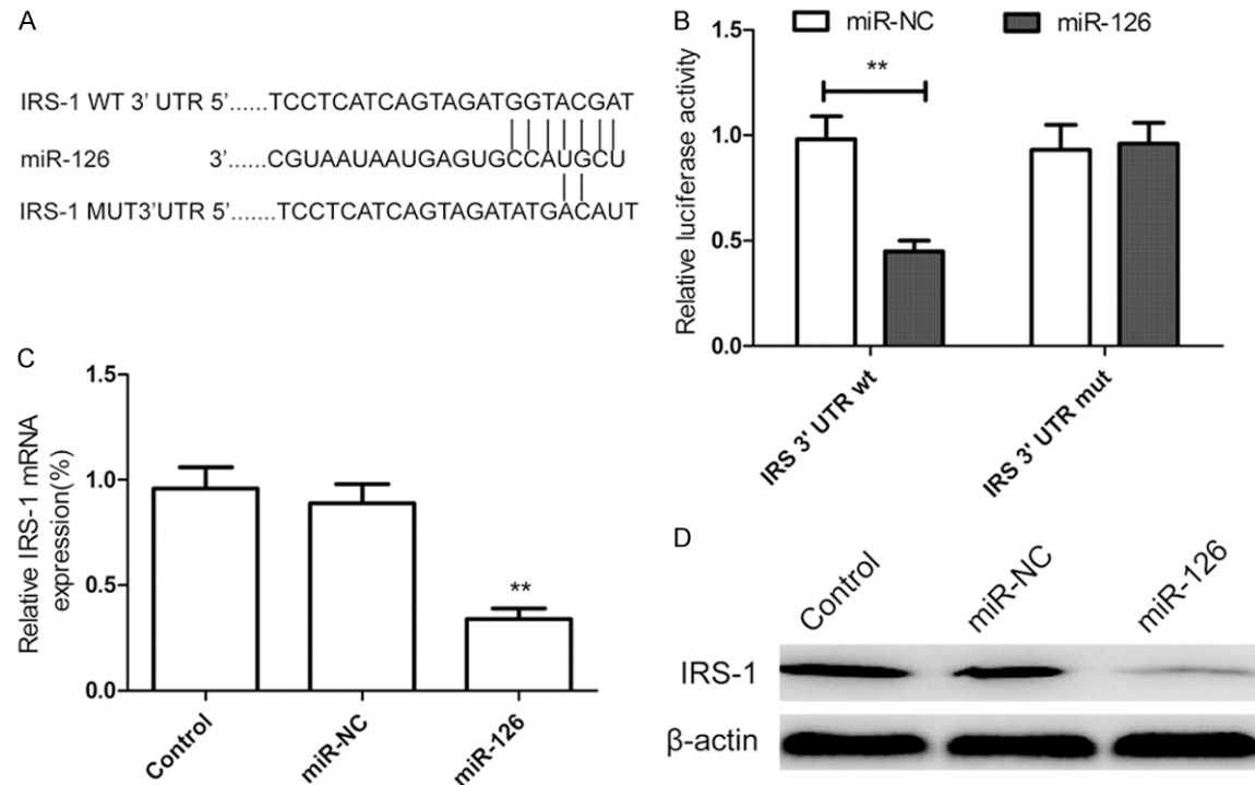
Figure 3. miR-126 targets the 3'-UTR of IRS-1 and down-regulates its expression. A. The predicted binding sites for miR-126 in the 3'UTR of IRS-1 and the mutations in the binding sites are shown. B. U87 cells were transfected with the wild type or mutated version of the luciferase-IRS 3'-UTR reporter vector as well as the miR-126 mimics or miR-NC for 48 h, then luciferase reporter assay were performed. C. Measurement of IRS-1 mRNA expression levels in U87 cells by qRT-PCR after transfected with the miR-126 mimics or miR-NC. The endogenous expression levels of the \beta -actin mRNA were used for normalization. D. Measurement of IRS-1 expression levels in U87 cells by western blot analysis after transfected with the miR-126 mimics or miR-NC. The endogenous expression levels of the \beta -actin protein were used for normalization. * P < 0.05 , ** P < 0.01 versus control.
