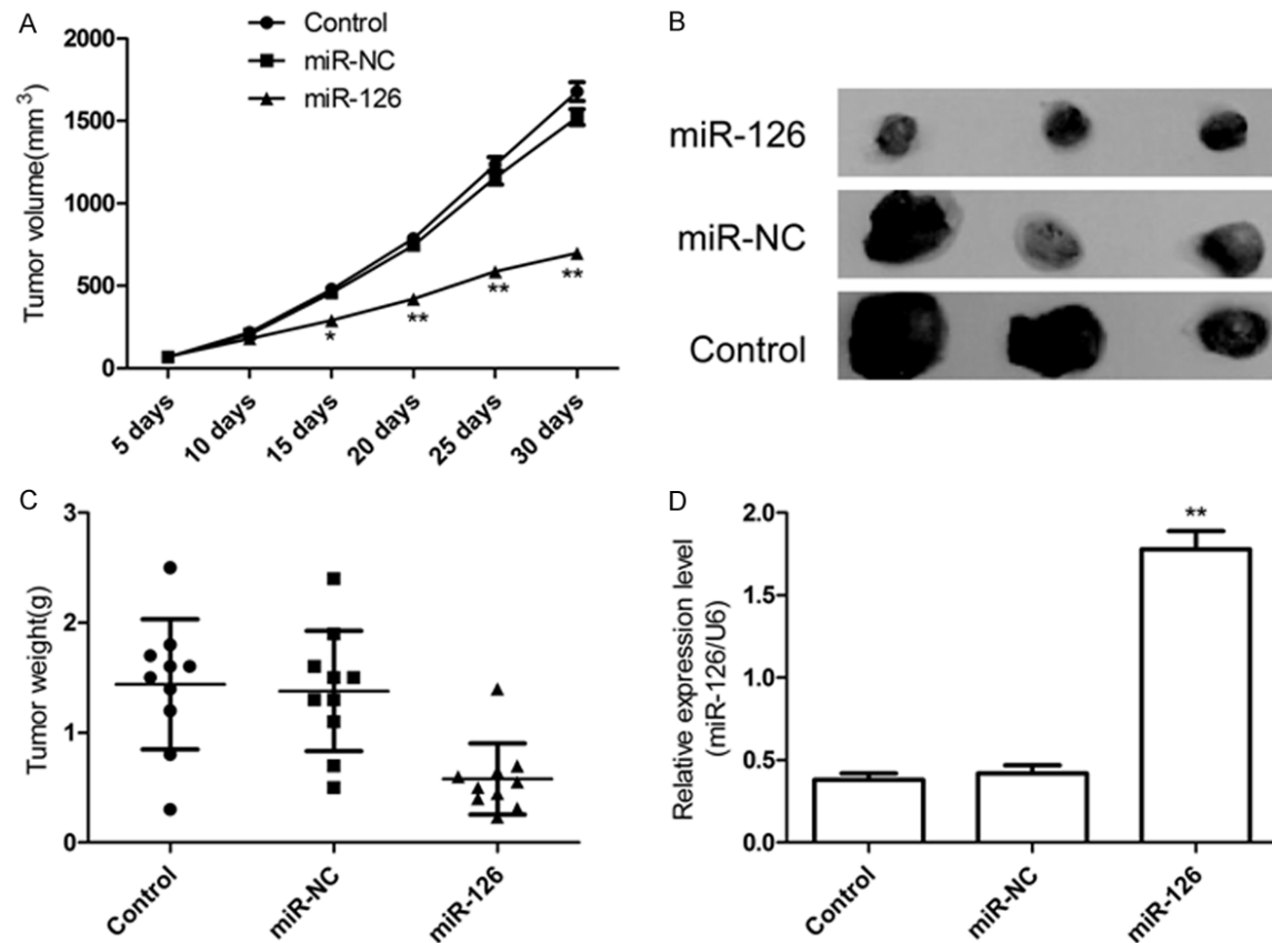
Figure 5. miR-126 suppressed tumor growth of glioma in a xenograft model. A. Growth curves for tumor volumes in xenografts of nude mice were established based on the tumor volume measured every five days until 30 days. B. Photographs of tumor tissue with different group at day 30. C. Tumor weights of different group at day 30. D. miR-126 level in tumor tissues of different group was determined by qRT-PCR. *P < 0.05, **P < 0.01 versus control group.
