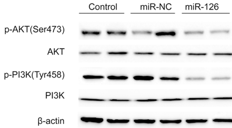
Figure 4. Effects of miR-126 on activation of PI3K/AKT signaling pathways in glioma cells. PI3K, p-PI3K, AKT, p-AKT protein expression levels in U87 cells were determined by western blot after transfected with miR-126 mimic or miR-NC. The endogenous expression levels of the \beta -actin protein were used for normalization.
