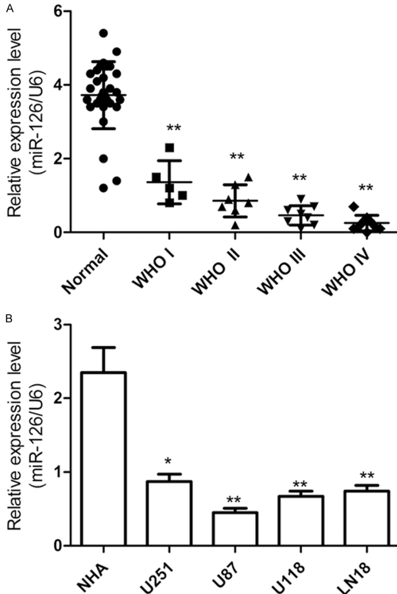
Figure 1. miR-126 was down-regulated in human glioma tissues and cell lines. A. Real-time quantitative RT-PCR (qRT-PCR) analysis of miR-126 expression in glioma tissues from different grades and adjacent normal brain tissues. U6 was used as loading control. B. Real-time quantitative RT-PCR (qRT-PCR) analysis of miR-126 expression in four glioma cell lines and primary normal human astrocytes (NHA). *P < 0.05 and **P < 0.01.
